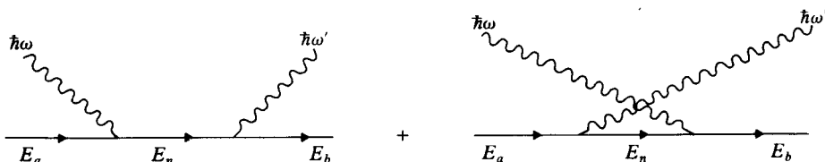
10.5 The two second-order terms in scattering of photons by atomic systems.
